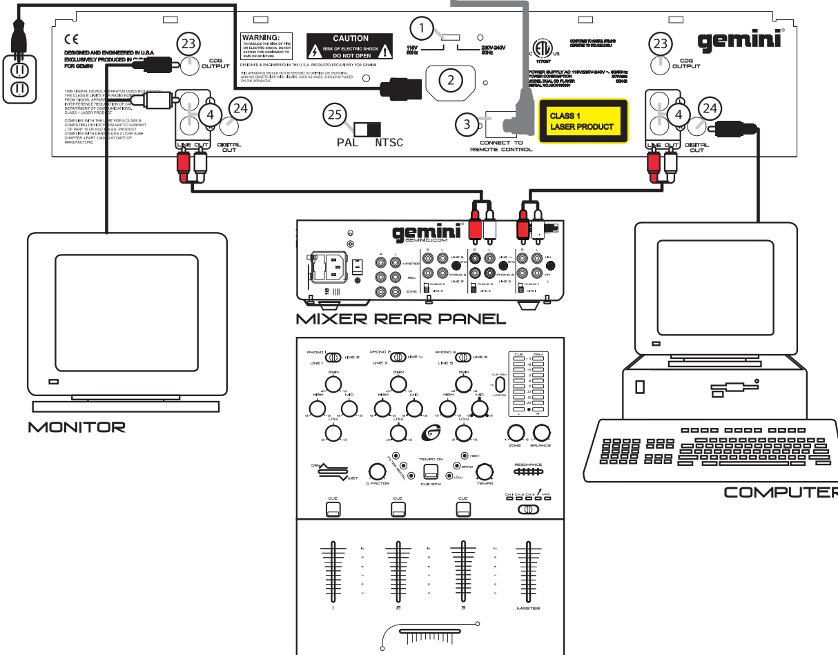
REAR MAIN
